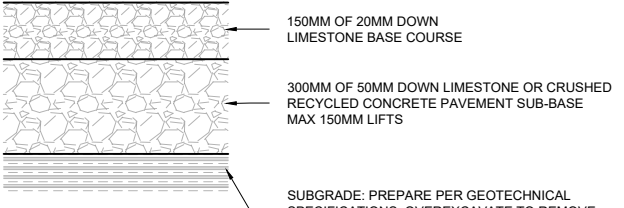
D HD GRAVEL STRUCTURE NTS
