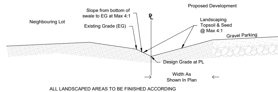
A TYPE 1 SWALE NTS
