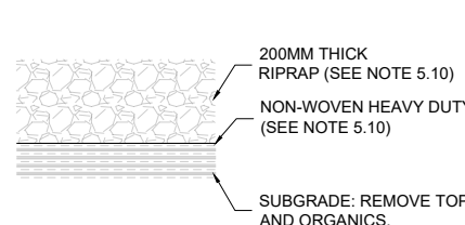
C RIPRAP STRUCTURE NTS
