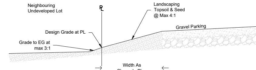
B TYPE 2 SWALE NTS
