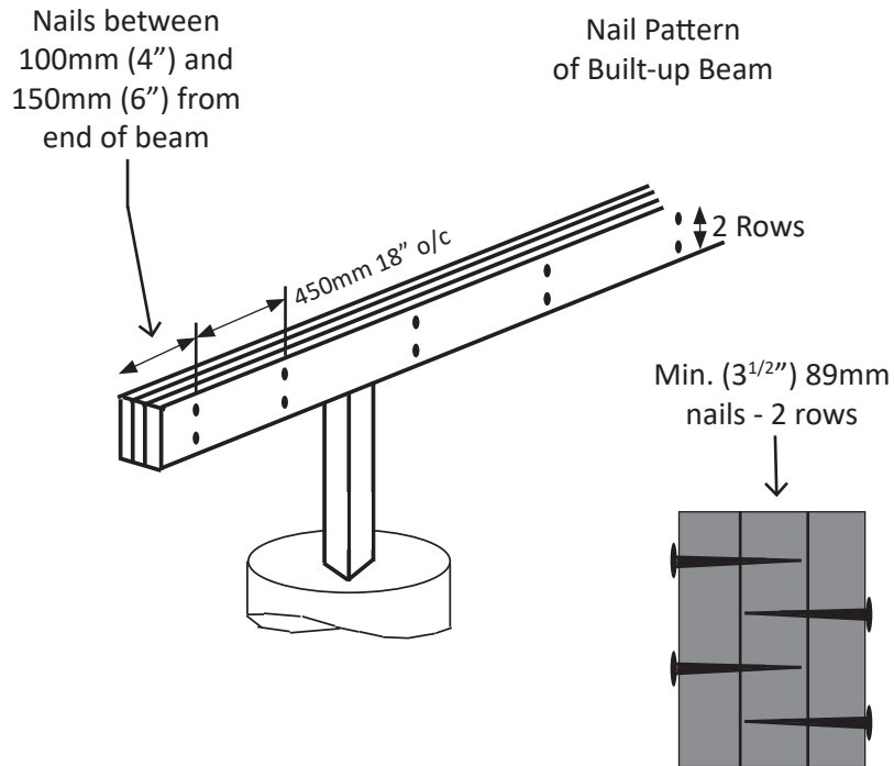
Figure 6a: Laminations
